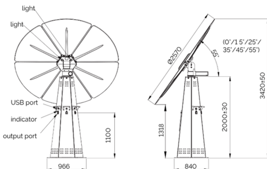
Figure 1. Dimension and diameter HEX600
