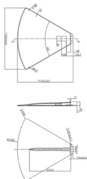
Figure 2. Dimension of solar panel
